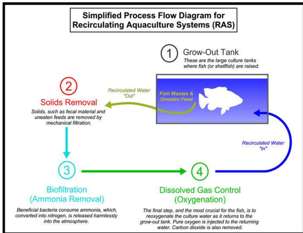
Figure 1. Structure of RAS (Source: Blue ridge aquaculture, 2017).
