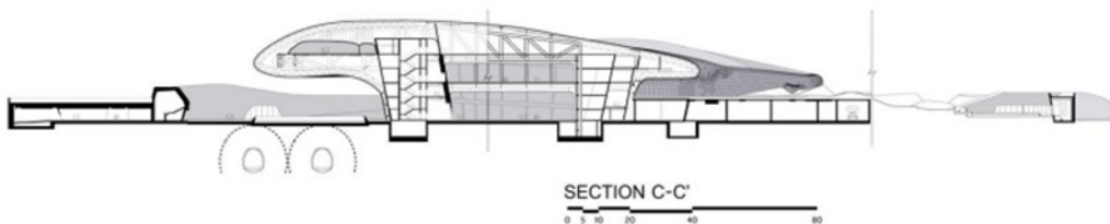
Figure 4.18: Dongdaemun Design Plaza section C-C'. 133
